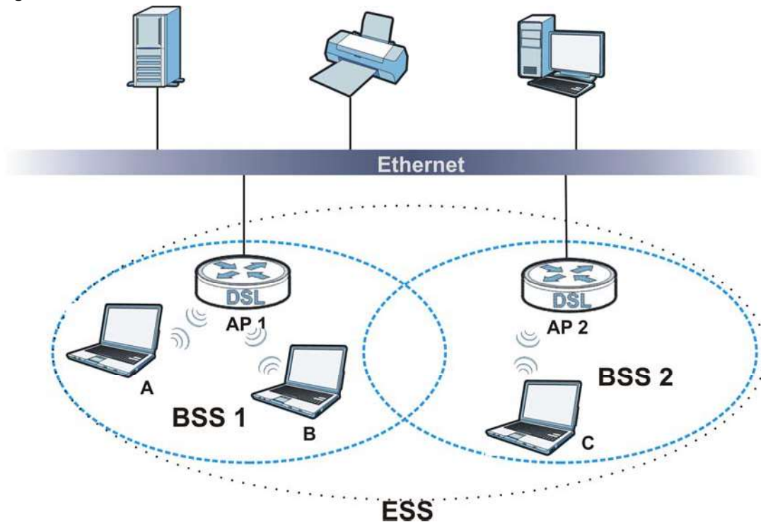
Figure 195 Infrastructure WLAN
