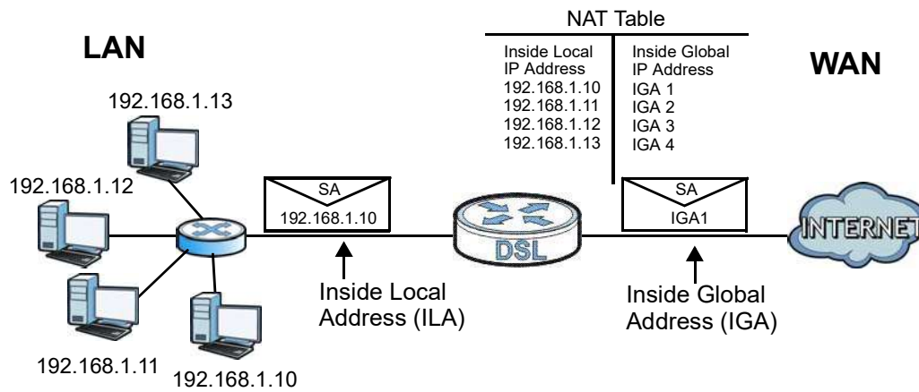
Figure 83 How NAT Works
