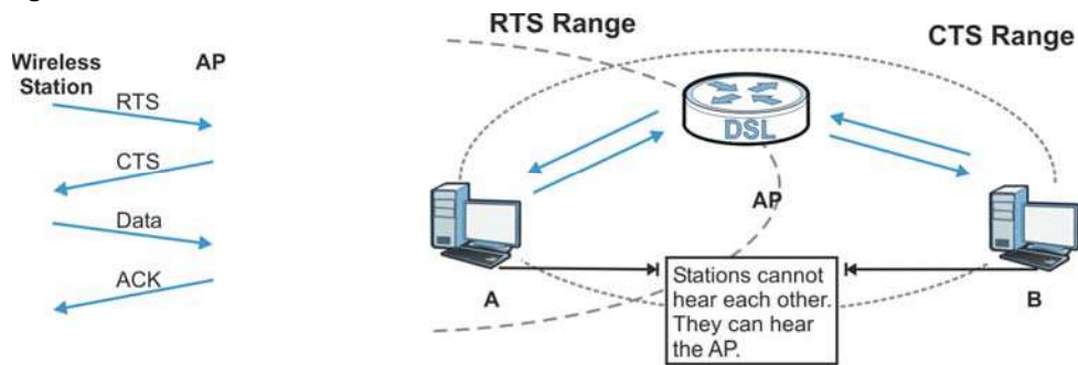
Figure 196 RTS/CTS
