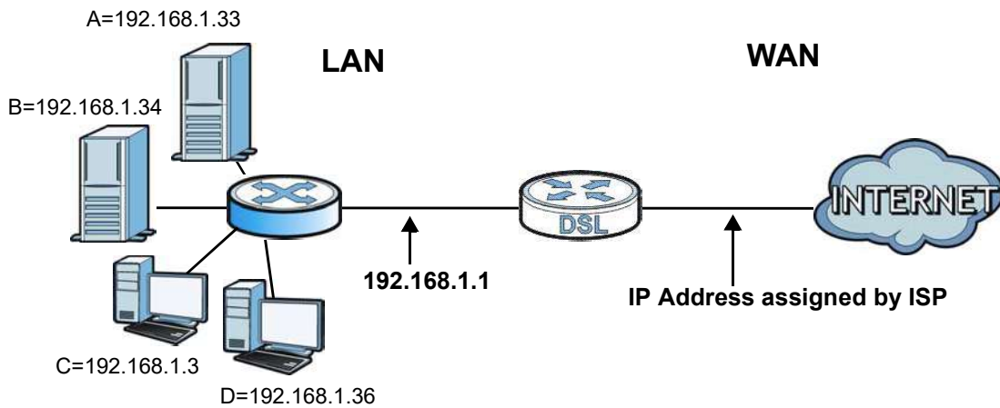
Figure 71 Multiple Servers Behind NAT Example
