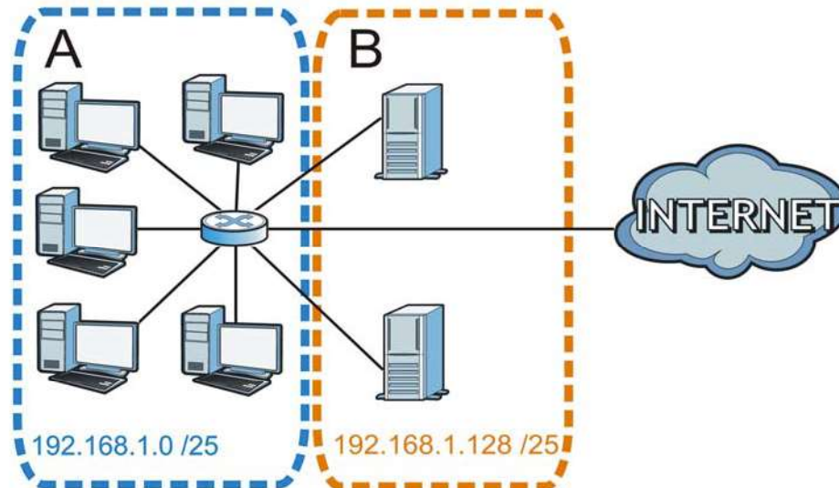
Figure 182 Subnetting Example: After Subnetting
